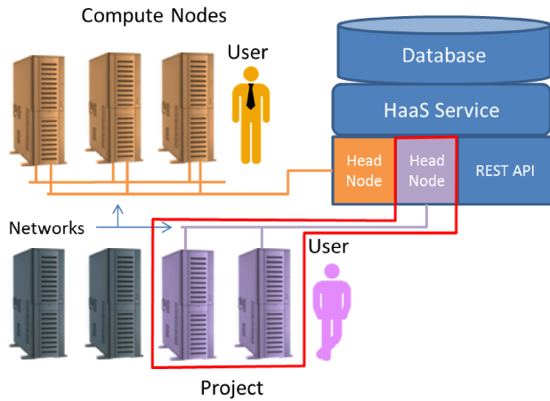
Fig. 1. Diagram of major HaaS components showing two isolated projects. One is managed by a professional (top; orange) while the other is managed by someone more casual (bottom; purple). A project represents a collection of resources and is managed by groups which contain individual users . Projects can contain allocated compute nodes , a head node and networks . Compute nodes represent bare metal systems, whereas a head node can either be a virtual or physical system from which provisioning or other management software may be run. Networks are generic methods of communications that connect compute nodes through a node's NIC to a particular switch. The HaaS Service tracks state and processes client requests to configure resources.
