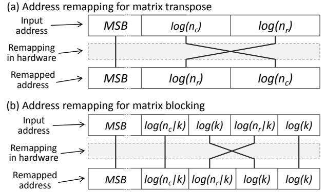
Fig. 5. Address remapping in hardware for the memory layout transforms matrix transpose and matrix blocking ( n_r \times n_c element matrix, k \times k blocks).
